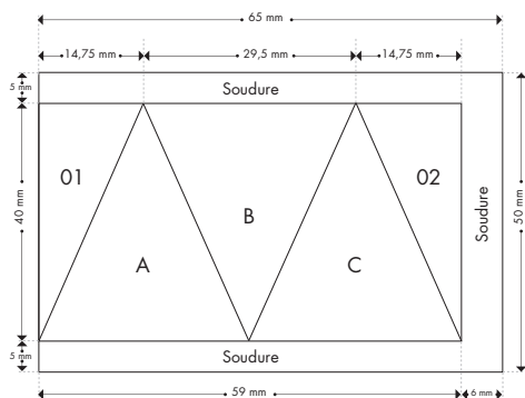
STRUCTURE DES BERLINGOTS TRANSPARENTS
