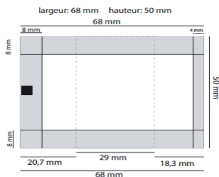
STRUCTURE DES BERLINGOTS TRANSPARENTS
